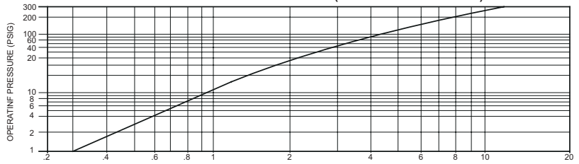
MODEL 3710 VENTING CAPACITIES (2mm ORIFIC DIAMETER)
